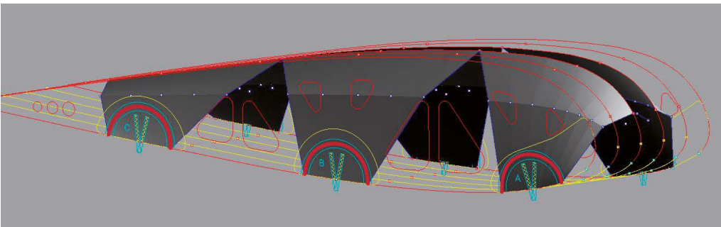
One of the precursors to rods: the designer Gibus placed them around the anchor points on the AirCross U3.
