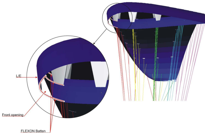
In 2002, Apco were already using 'Flexon Battens' on the Keara.
