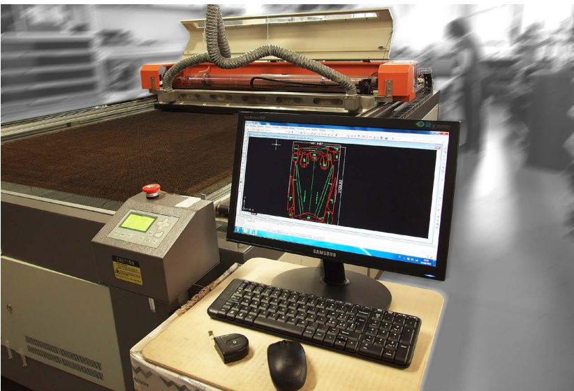
Computerised cutting at Woody Valley the harness manufacturer, using the same principle as for the paraglider profiles. (Photos: Woody Valley)
