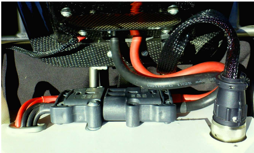
The two connections which link the battery to the motor: one for 'data' (black woven cable) the other for power (thick red and black electric cables).
